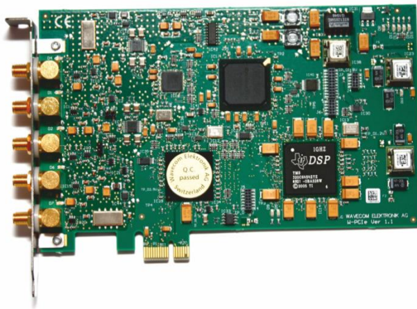
W-PCle card.
